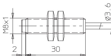
E2EL-X2M□-L 2M
