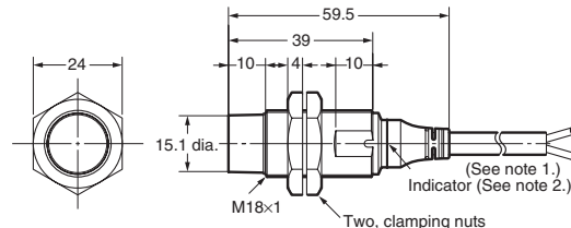
E2A-M18KN16-WP-□□/E2A-S18KN16-WP-□
