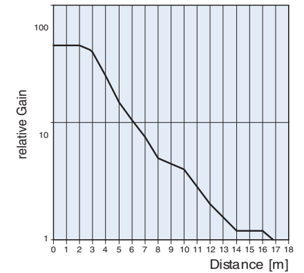
Through-beam Models (axial) E3F2-10□
