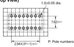
PCB Dimensions (Top View)
