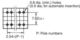
Mounting holes (top view)
