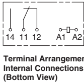
Input circuit
