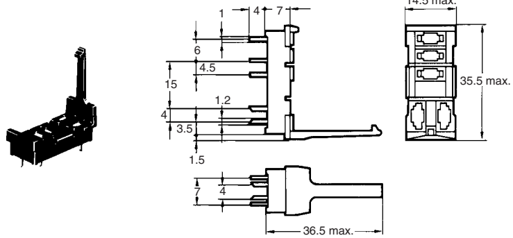
P2R-05P (1-pole)
