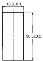
Recommended thickness of the panel is 1.6 to 2.0 mm
