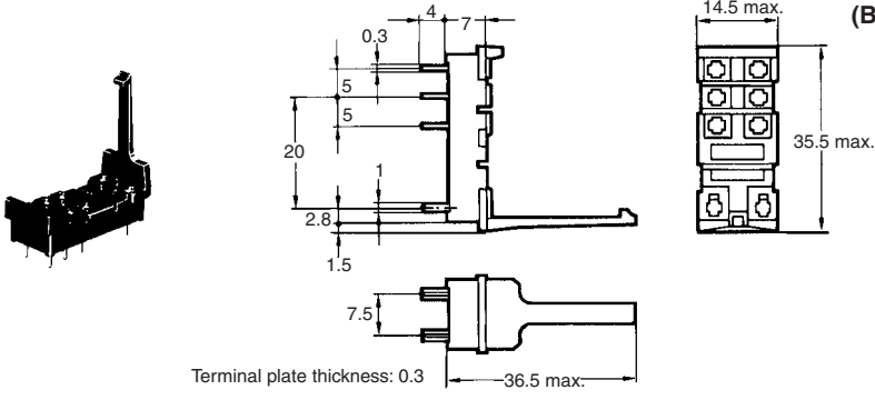
P2R-05A (1-pole)
