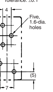
Mounting Holes
